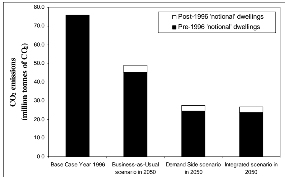
Figure 3 Total CO 2 emission predictions for modelled scenarios in the year 2050 (source: Johnston et. al., in press)
