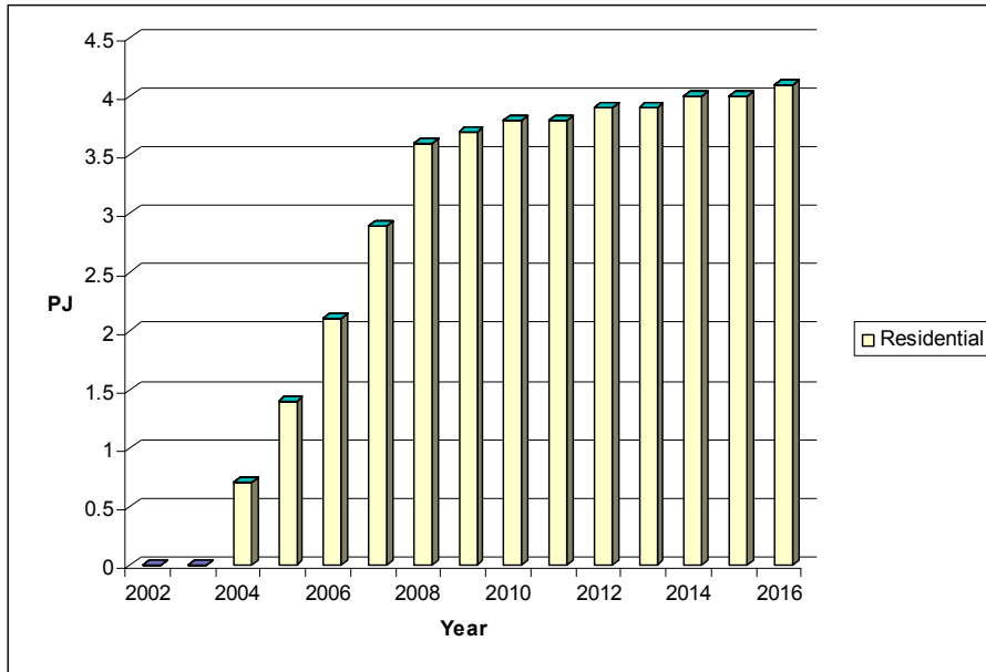
Figure 8: Residential solar hot water heaters
