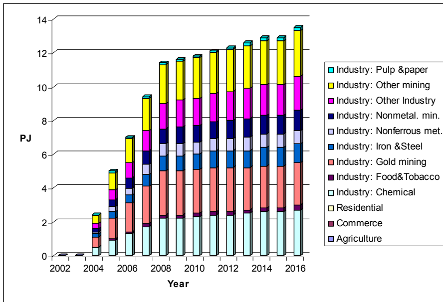
Figure 3: Compressed air saving program
